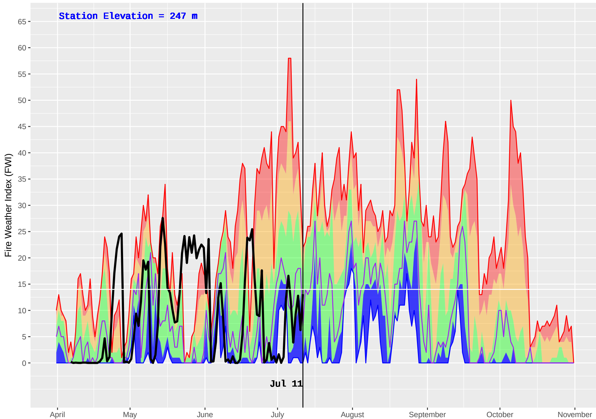
FORD MOUNTAIN (1144) : Historical (2012–2016) and Current (2018) Noon Fire Weather Index (FWI)
