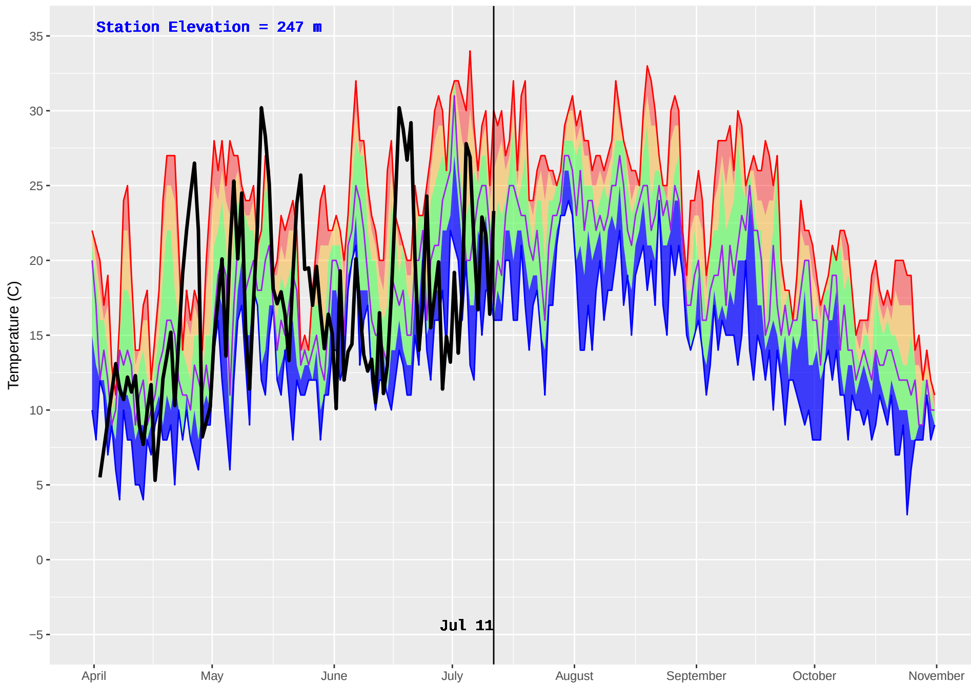
FORD MOUNTAIN (1144) : Historical (2012–2016) and Current (2018) Noon Temperature
